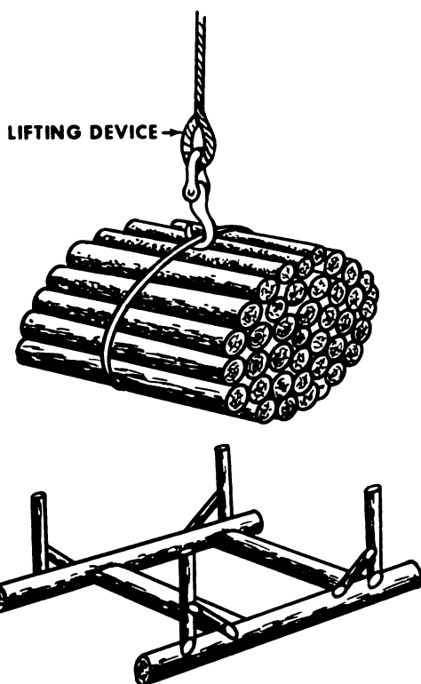
2 HANDLING THE LOADED STEEL HOOP
